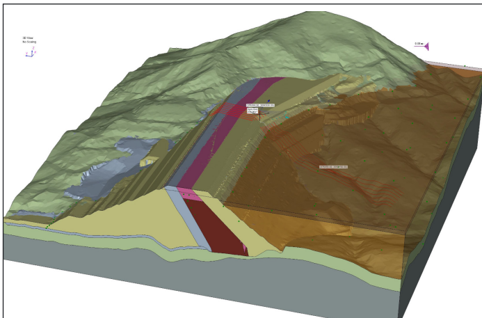
Safety and efficiency of a mine tailings facility is improved by using PLAXIS LE.
